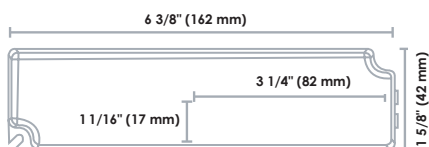
LED Driver
